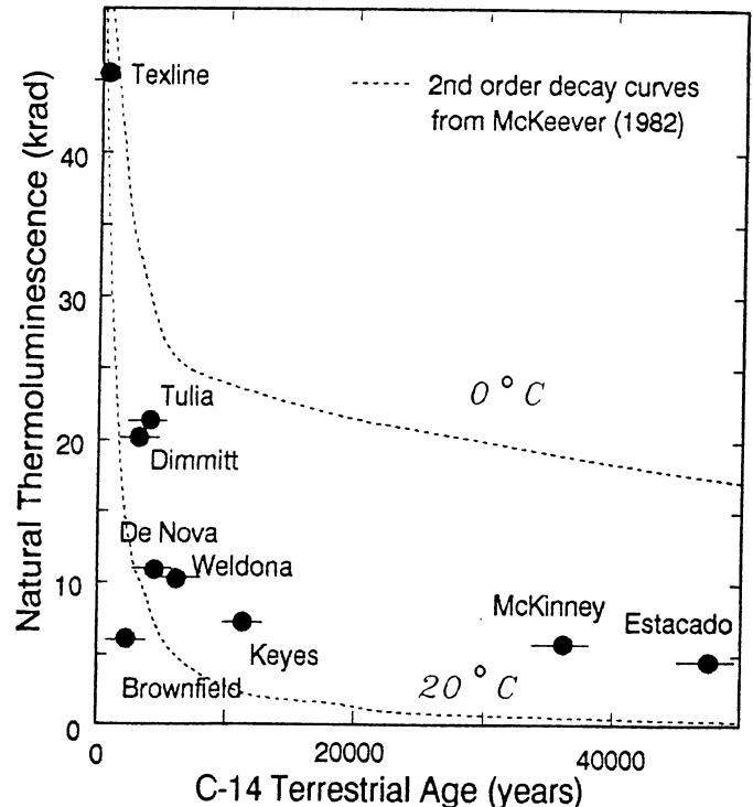
Fig. 1. Natural TL compared with terrestrial ages determined by AMS measurements for 14 C.
