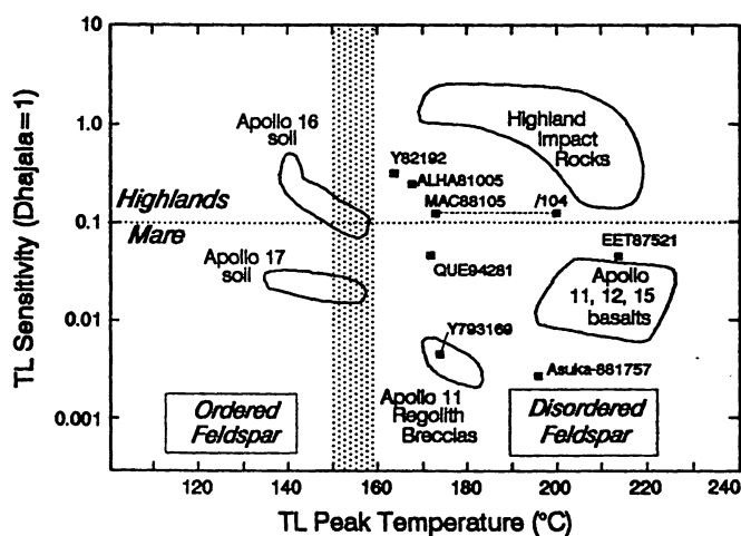
Fig. 1. TL properties of highland and mare lunar meteorites compared with various Apollo samples.
