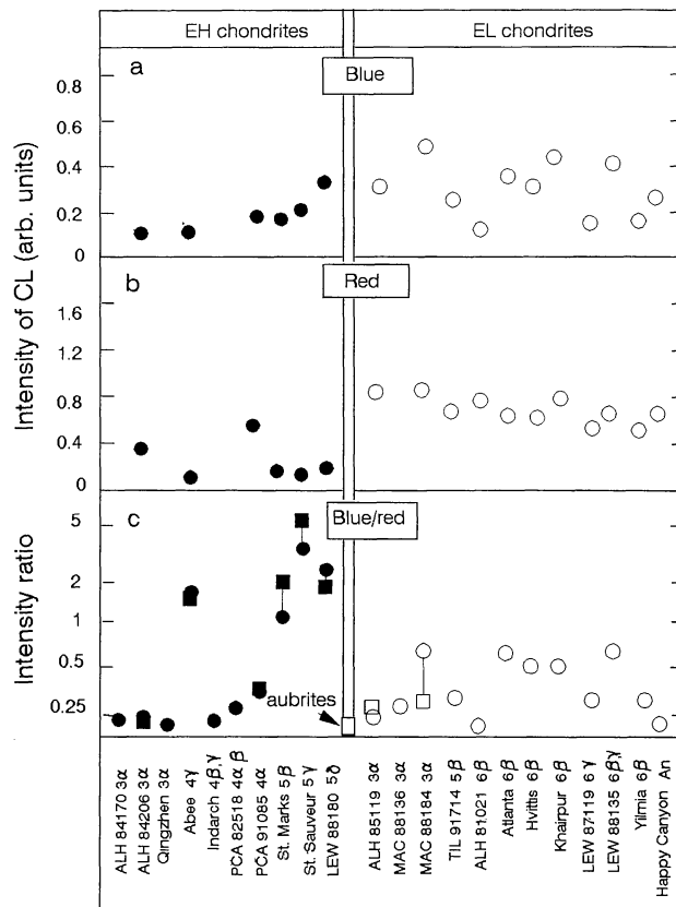
FIG. 3. Quantitative data for the bulk CL properties of enstatite chondrites determined from CL spectra similar to those of Fig. 2. (a) The intensity of the blue peak increases with textural and mineralogical type in the EH chondrites, but the EL chondrites display no systematic trends. (b) The intensity of the red peak does not appear to vary systematically with textural and mineralogical type in either class but is a factor of ~2 higher in the EL chondrites. (c) The ratio of the intensity of blue and red peaks increases with type for the EH chondrites and is independent of type in the EL chondrites. It is higher for equilibrated EH chondrites than the other enstatite meteorites. Blue/red ratios obtained by point counting the CL images are also shown as squares and connected to the spectral data by tie lines. Unless otherwise indicated, on all our figures 1\sigma experimental precisions are approximately twice the size of the symbols. Also shown is the range of blue to red spectral peak ratios measured for aubrites by Geake and Walker (1966).
