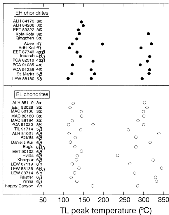
FIG. 5. Plot to compare the induced thermoluminescence peak temperatures of enstatite chondrites. Except for EH3 \alpha chondrites, enstatite chondrites show peaks at ~140 °C and ~300 °C in the glow curve. In a few instances, the ~140 °C peak can be resolved into two peaks (at ~120 °C and ~170 °C). The EL6 \beta chondrites show considerable scatter in the position of the high temperature peak.
