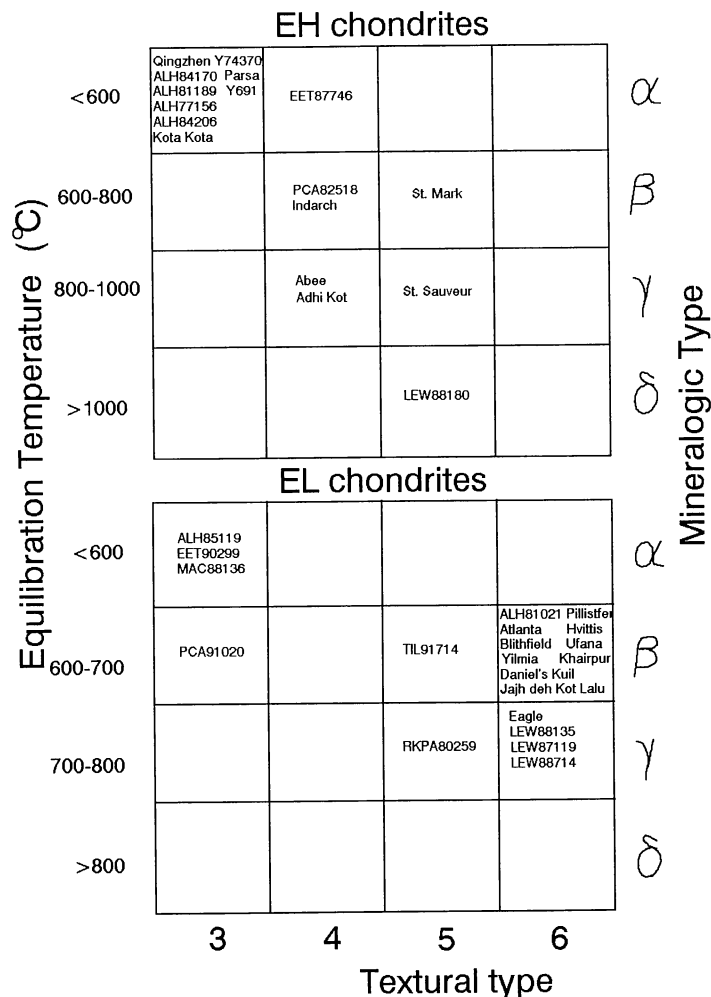
FIG. 8. Distribution of enstatite chondrites over mineralogic ( \alpha - \delta ) and textural (3-6) types with suggested equilibration temperatures that are based on the pyroxene structure.
