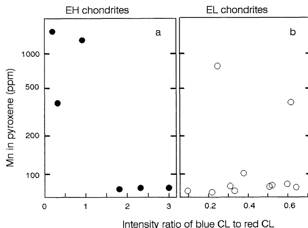
FIG. 7. Plot to compare the Mn content in pyroxene in enstatite chondrites with the intensity ratio of blue CL to red CL obtained from the spectra. (a) EH chondrites show a decrease in the Mn content of the enstatite with increasing blue CL to red CL ratio. (b) EL chondrites display no obvious trend.
