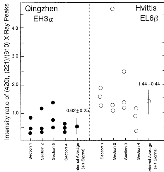
FIG. 1. Plots of the ratio of the 420, 221 doublet to the 610 singlet in the x-ray diffraction pattern of two enstatite chondrites. Four sections of each sample were prepared, and each was scanned three times. According to Pollack and Ruble (1964), the doublet is more intense than the singlet for ordered enstatites while the reverse is true of disordered enstatite. The internal average (average ignoring the highest and lowest points) is shown for the peak height ratios of each meteorite.
