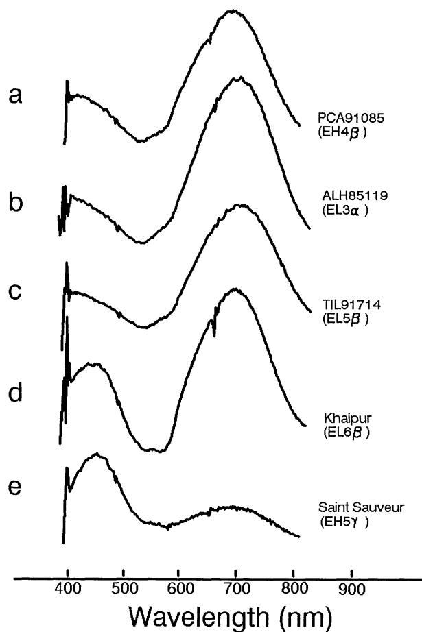
FIG. 2. Representative cathodoluminescence spectra of bulk samples of enstatite chondrite. Baselines have been displaced vertically for clarity. Little-metamorphosed chondrites of both the EH (a) and EL (b) classes have spectra with strong red (~700 nm) and weak blue (~450 nm) CL peaks. Metamorphosed EL chondrites (c and d) also have spectra with strong red peaks, but the blue CL peaks can be of almost comparable intensity to the red CL peak. Metamorphosed EH chondrites have strong blue and weak red CL peaks. These spectra are consistent with CL images in Plate 1.
