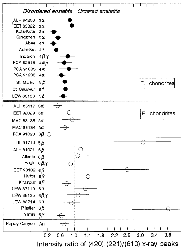
FIG. 4. The x-ray diffraction data for enstatite chondrites. According to Pollack and Ruble (1964), the relative intensity of the (420), (221) doublet and the (610) peak is a measure of the stacking order in the enstatite; the doublet peak is stronger than the singlet in ordered orthopyroxene but weaker for disordered orthopyroxene. All of the EH chondrites and the EL3 \alpha chondrite appear to contain disordered enstatite, while eight of twelve EL6 chondrites contain ordered enstatite.
