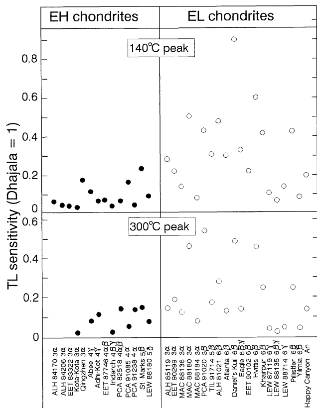
FIG. 6. Plot comparing the thermoluminescence sensitivities of enstatite chondrites. The \sim 140^\circ\text{C} and the \sim 300^\circ\text{C} peaks behave similarly, suggesting that they are caused by the same luminescent minerals and activators. Since our TL apparatus is biased towards blue wave lengths, the variations in TL sensitivity shown by enstatite chondrites resemble those of the blue CL intensity.
