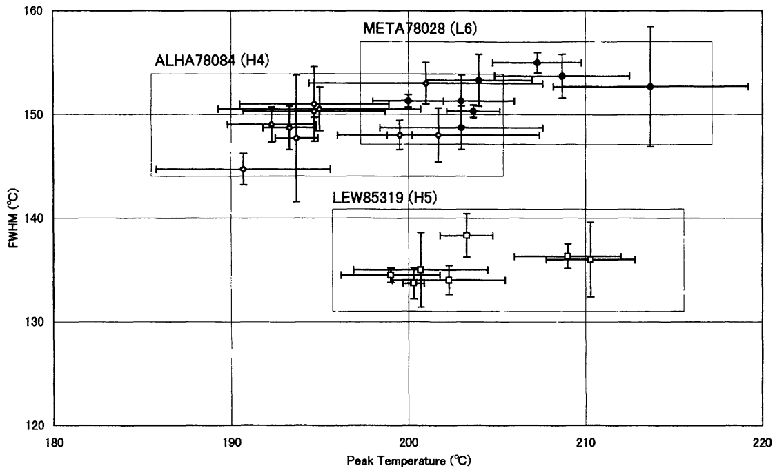
Fig. 8. TL peak width vs. TL peak temperature for three large Antarctic ordinary chondrites. The rectangles correspond to regions in which peak temperature varies by 20°C in peak temperature and peak width by 10°C.
