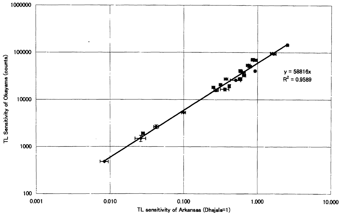
Fig. 2. Plot comparing the TL sensitivities of ten equilibrated and fifteen unequilibrated ordinary chondrites measured at the University of Arkansas and Okayama University of Science. The TL sensitivities of induced TL of Arkansas are normalized by that of Dhajala, while the Okayama data are effectively normalized to applied dose.
