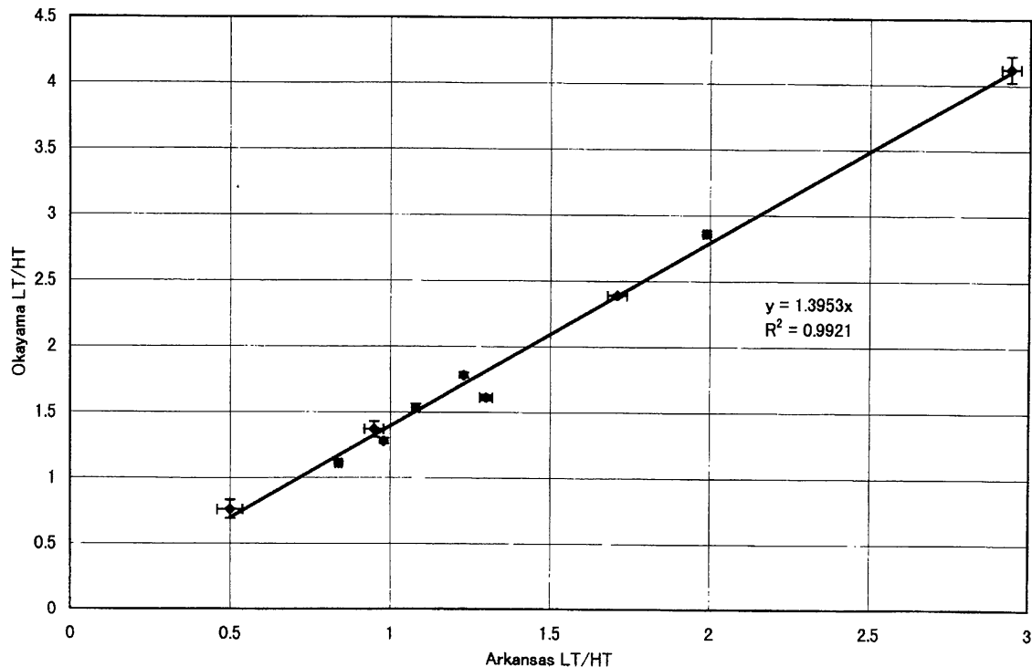
Fig. 1. Plot comparing the natural LT/HT ratio of ten equilibrated ordinary chondrites measured at the University of Arkansas and Okayama University of Science. The LT is intensity of low temperature glow peak and the HT is intensity of high temperature glow peak.
