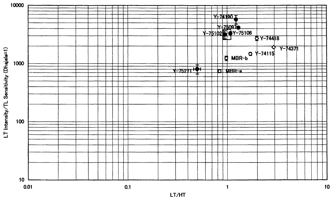
Fig. 9. Same as Fig. 7 but for ten equilibrated ordinary chondrites from the Japanese Antarctic meteorite collection.
