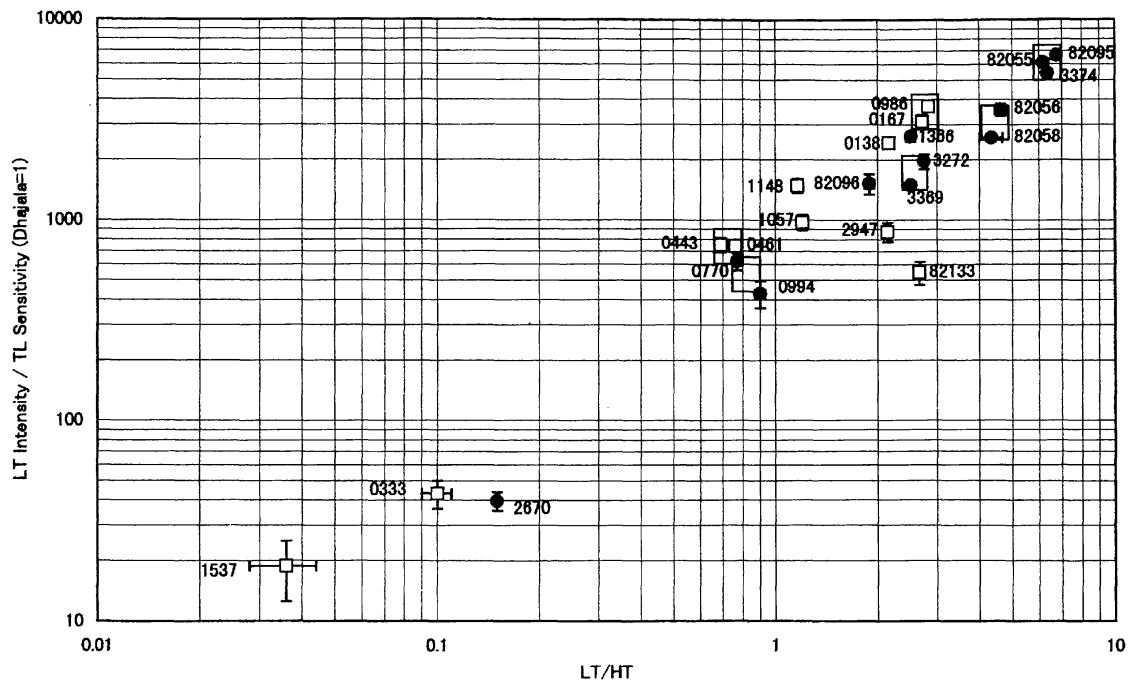
Fig. 10. Ratio of the natural TL signal (raw data as number of counts) to the Dhajala-normalized TL sensitivity vs. natural TL peak height ratio for twenty-eight unequilibrated ordinary chondrites from the Japanese Antarctic meteorite collection. The rectangles correspond to regions in which LT intensity/TL sensitivity varies by a factor of 1.5 and LT/HT varies by 20%. Meteorites may be identified from Table 5, the last 4 or 5 numbers of the meteorites' names have been used. □: H3, ●: L3
