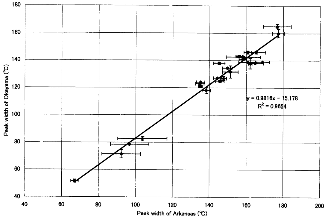
Fig. 4. Plot comparing the TL peak widths of ten equilibrated and fifteen unequilibrated ordinary chondrites measured at the University of Arkansas and Okayama University of Science.
