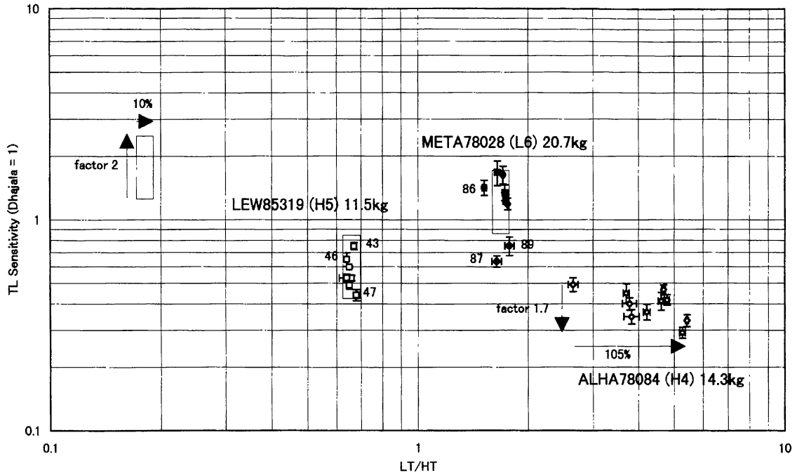
Fig. 5. Induced TL sensitivity vs. natural TL peak height ratio for three large Antarctic ordinary chondrites. The rectangles correspond to a factor of two in TL sensitivity and 10% in dose at 250°C. The number by each datum is the subsample number.
