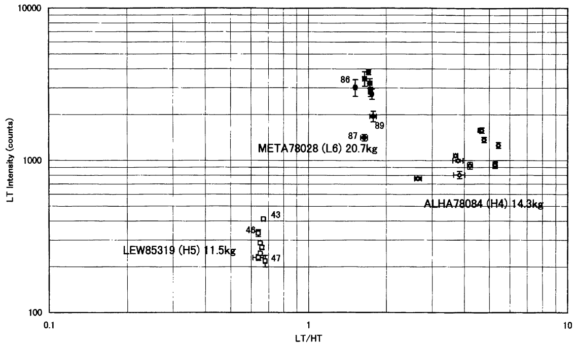
Fig. 6. Natural TL signal (raw data as number of counts) against natural TL peak height ratio for three large Antarctic ordinary chondrites. The number by each datum is the subsample number.
