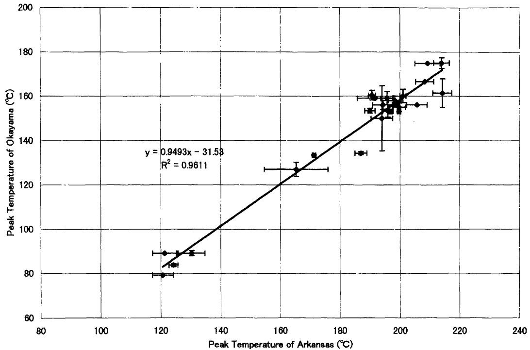
Fig. 3. Plot comparing the TL peak temperatures of ten equilibrated and fifteen unequilibrated ordinary chondrites measured at the University of Arkansas and Okayama University of Science.
