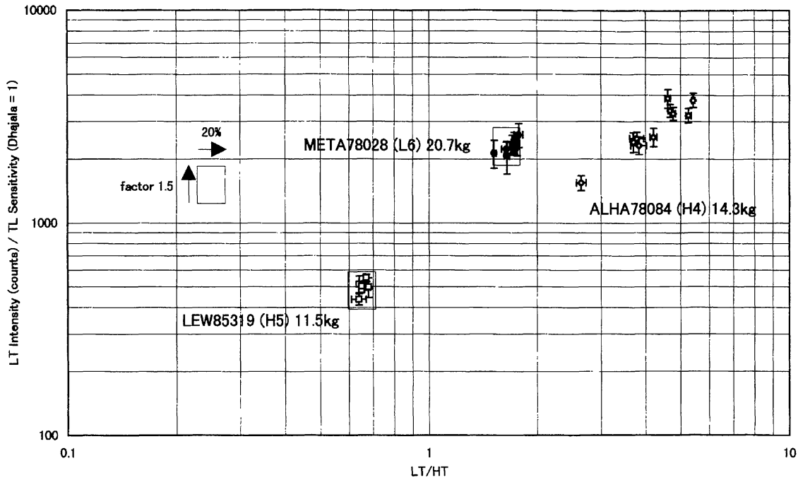
Fig. 7. Ratio of the natural TL signal (raw data as number of counts) to the Dhajala-normalized TL sensitivity vs. natural TL peak height ratio for three large Antarctic chondrites. The rectangles correspond to regions in which LT intensity/TL sensitivity varies by a factor of 1.5 and LT/HT varies by 20%. The number by each datum is the subsample number.
