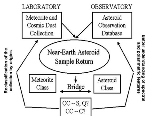
Fig. 1. The scientific rationale behind the Hera mission expressed as a logic flow chart. Only sample return from asteroids previously studied by remote observations and in situ/rendezvous measurements can bridge between the ground observations of minor bodies and laboratory analyses of meteoritic samples. (Courtesy Hajime Yano, ISAS.)
