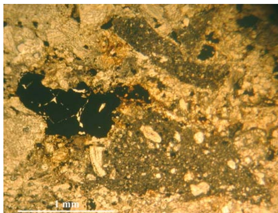
Fig. 3. Transmitted optical microscope image of detached fine-grained clasts forming part of the matrix of this meteorite. The scale in the lower left corner is 1 mm.
