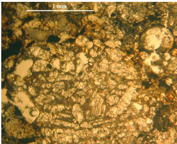
Fig. 2. Transmitted optical microscope image of a porphyritic chondrule of Cali meteorite. The scale in the upper left corner is 1 mm.
