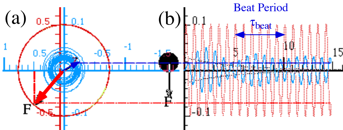
Fig. 3.2.10 Above Resonance (a)Response z -phasor lags \rho=170.2^\circ behind stimulus F -phasor. ( \omega_s=7.53, \omega_0=2\pi, \Gamma=0.2 ). (b) Time plots of Re z(t) and Re F(t)
