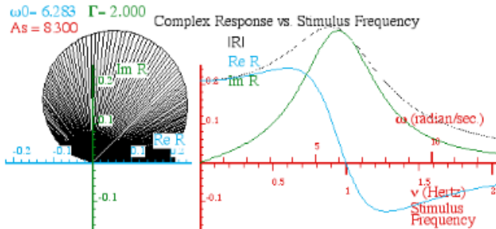
Fig. 3.2.14 Highly damped Lorentz-Green function plots with \Gamma=2.0 and \omega=2\pi .
