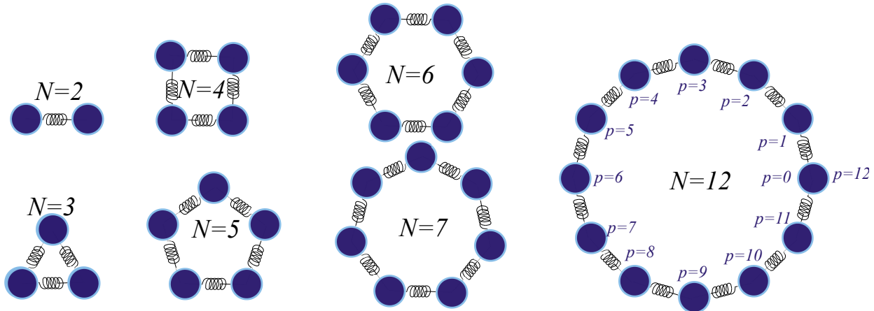
Fig. 3.8.4 N -Coupled Pendulums. (Viewed from above.)
