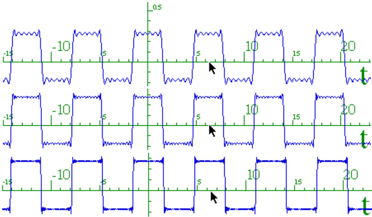
Fig. 3.6.3 Fourier series approximations to square wave stimulus up to k=9, 19, and 39 .
