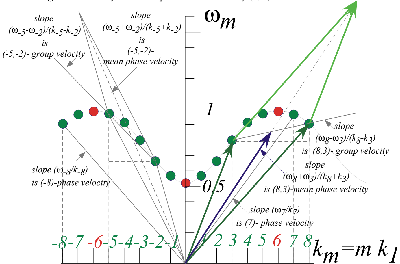
Fig. 3.8.9 Types of dispersion \omega(k) functions and geometry of phase and group velocity.
