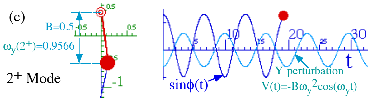
Fig. 3.7.5 symmetric 2^+ mode .
