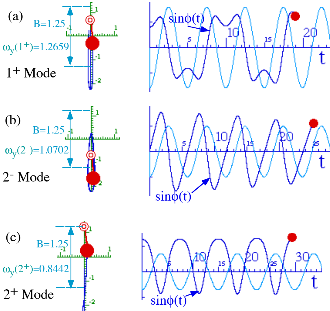
Fig. 3.7.8 Higher amplitude modes with hanging stability
