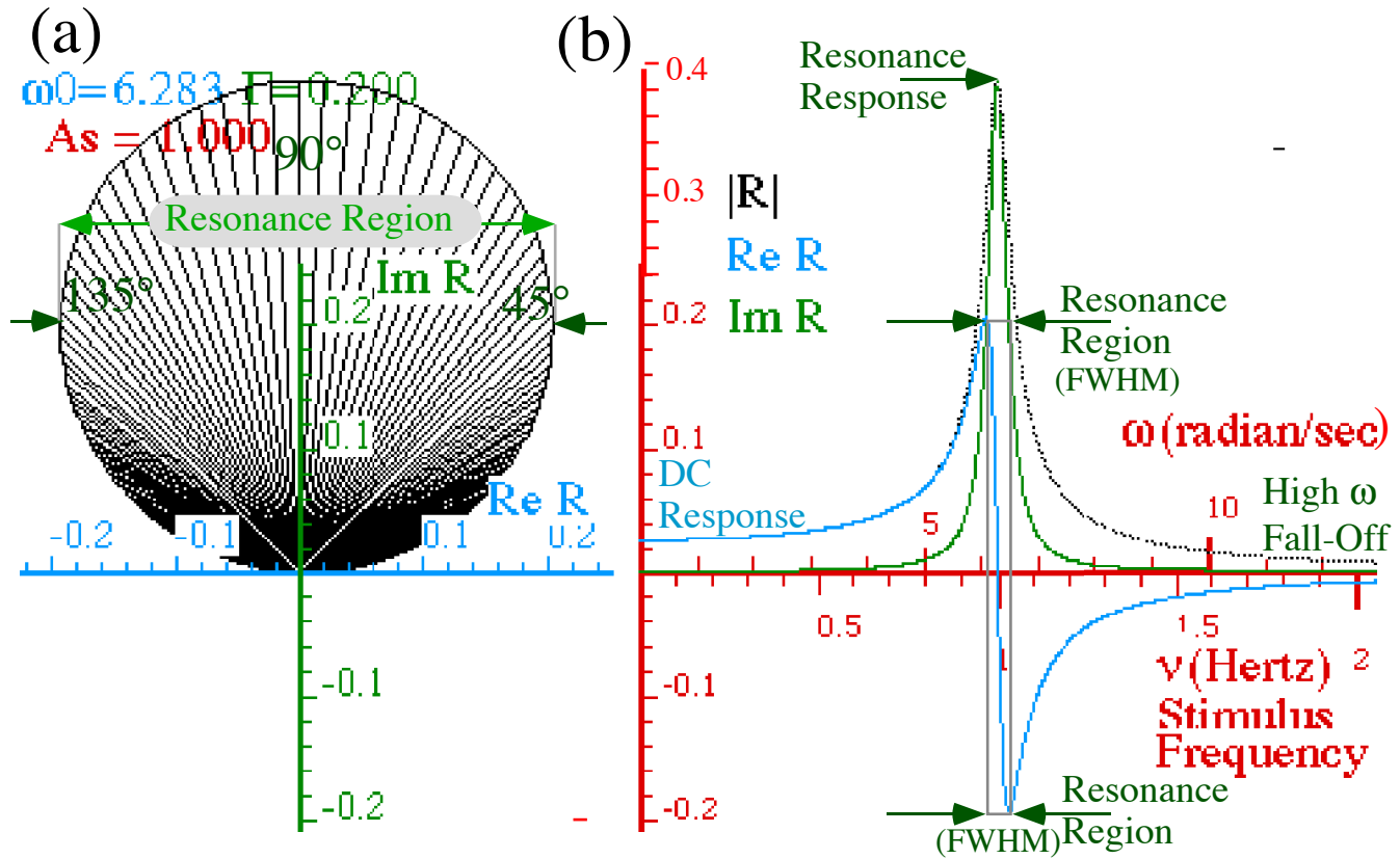
Fig. 3.2.6 Anatomy of oscillator Green-Lorentz response function plots
