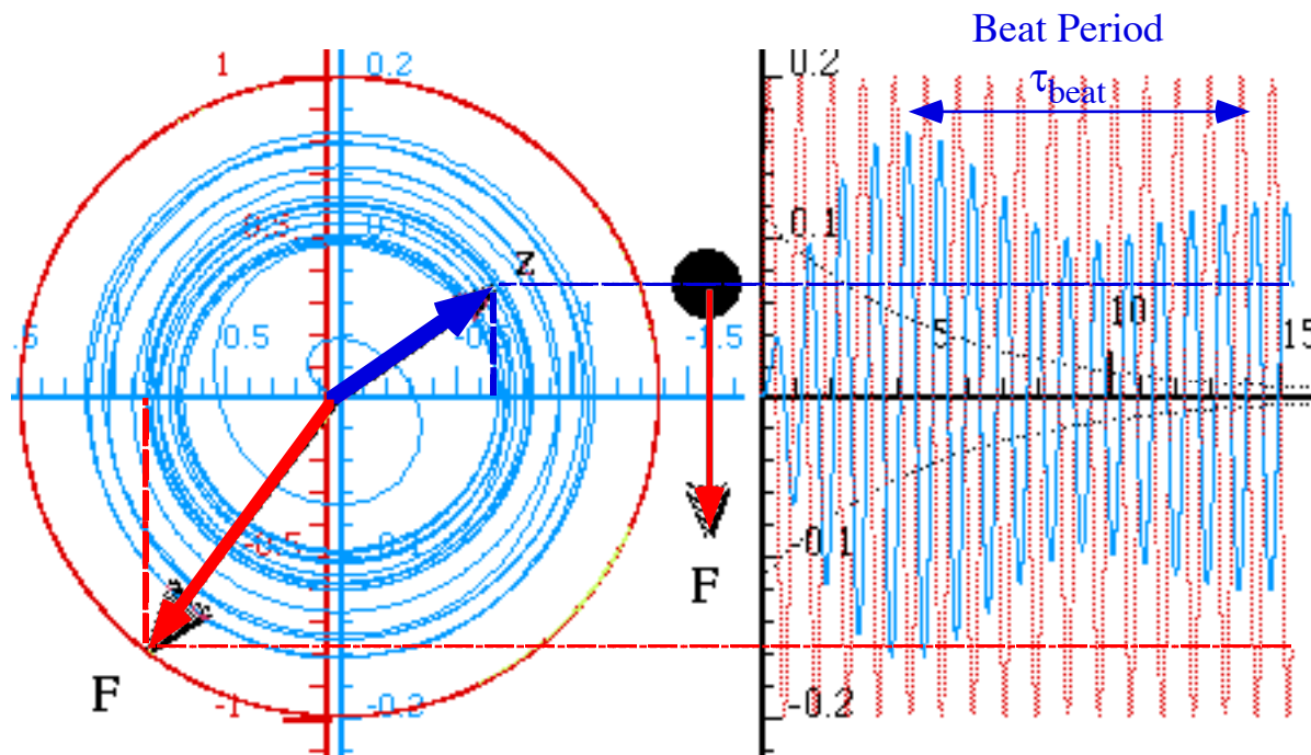
Fig. 3.2.11 Above Resonance (a)Response z -phasor lags \rho=161.6^\circ behind stimulus F -phasor. ( \omega_s=6.91, \omega_0=2\pi, \Gamma=0.2 ). (b) Time plots of Re z(t) and Re F(t)
