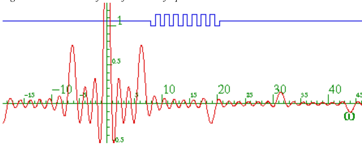
Fig. 3.6.10 Fourier transform of fifteen half square waves.
