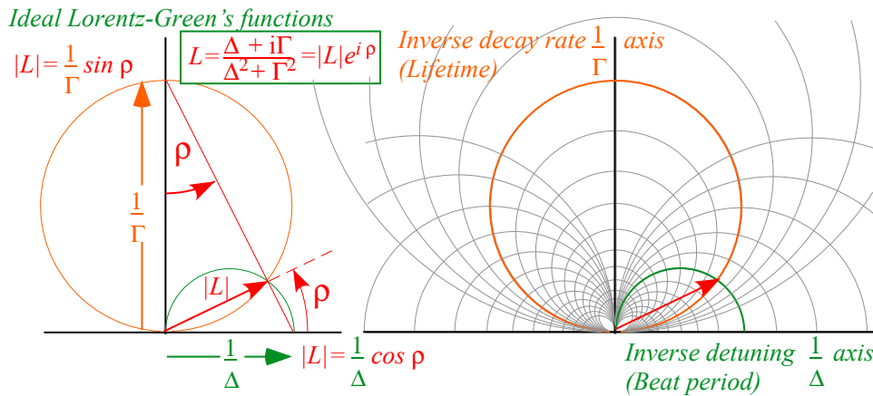
Fig. 3.2.13 Ideal Lorentzian in inverse rate space. (Smith life-time 1/\Gamma vs. beat-period 1/\Delta coordinates)
