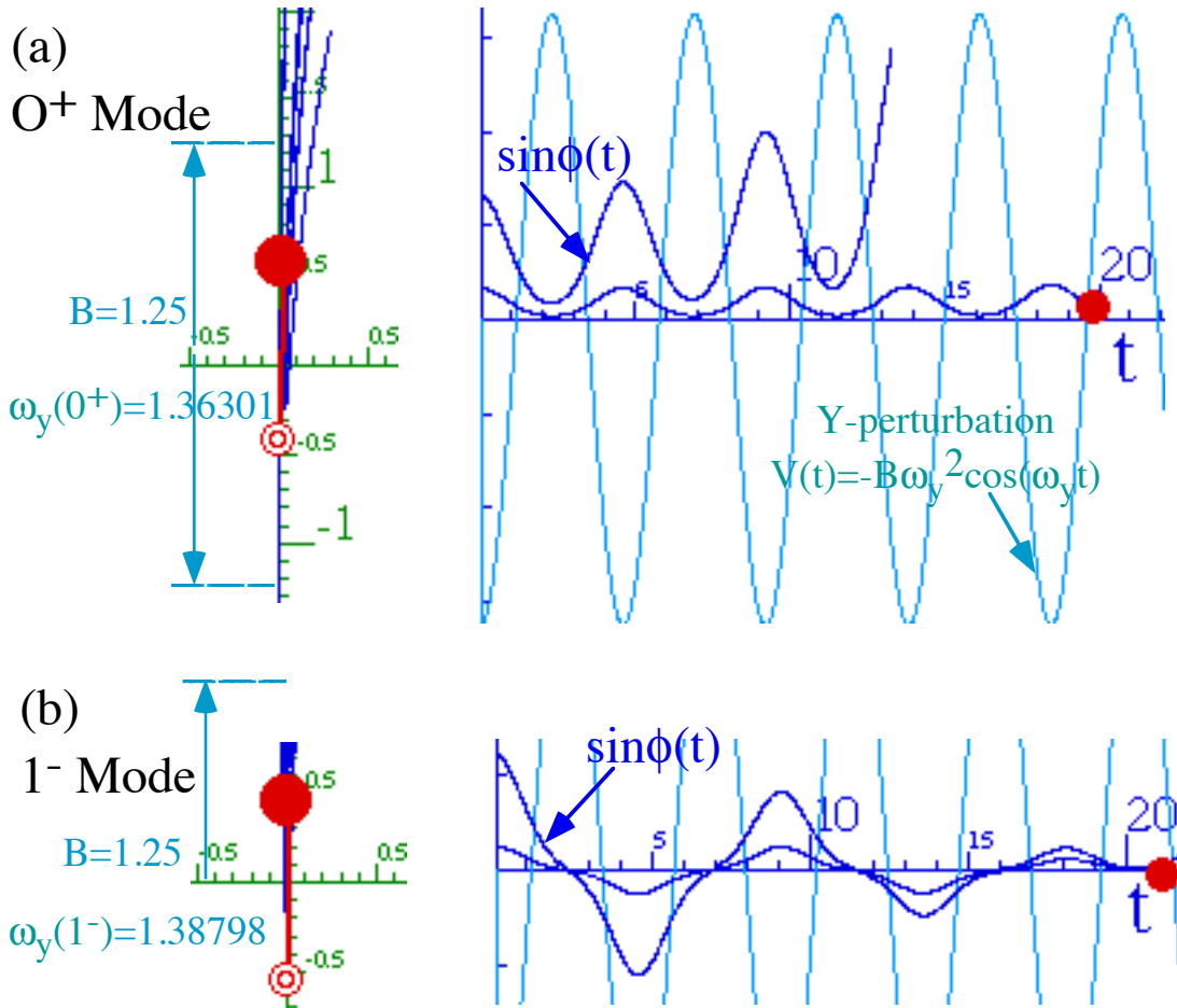
Fig. 3.7.7 Higher amplitude modes with inversion stability
