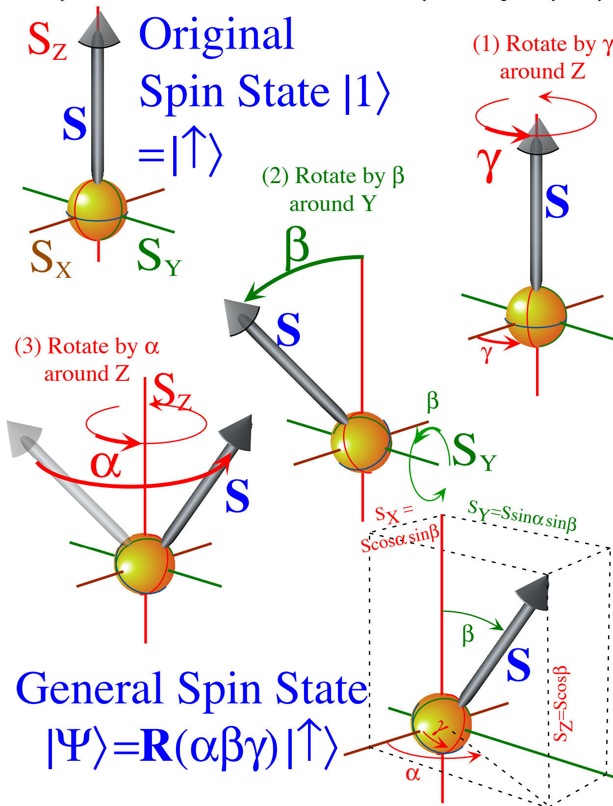
Fig. 3.4.3 The operational definition of Euler ( \alpha\beta\gamma )-angle coordinates is applied to a unit spin-state.
