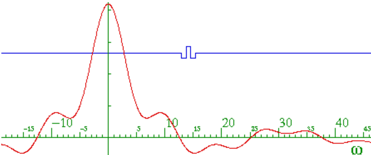
Fig. 3.6.8 Fourier transform of three half square waves.
