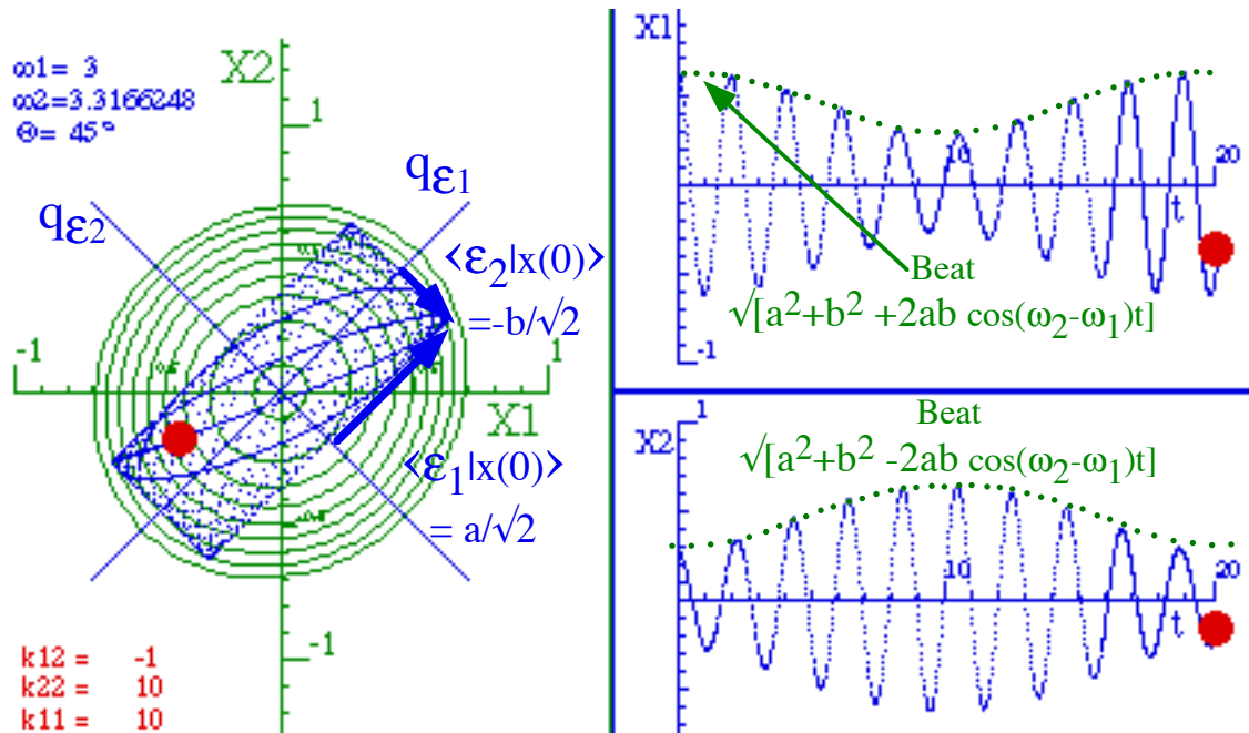
Fig. 3.3.10 Same as Fig. 3.3.9 but mode-1 magnitude a/\sqrt{2} is greater than b/\sqrt{2} for mode-2.
