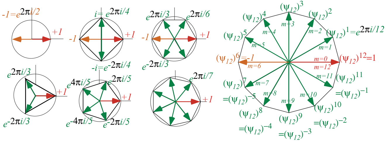
Fig. 3.8.5 N th -Roots of Unity. Collections of Fourier coefficients for discrete N=2,3,4,5,6,7, and 12.
