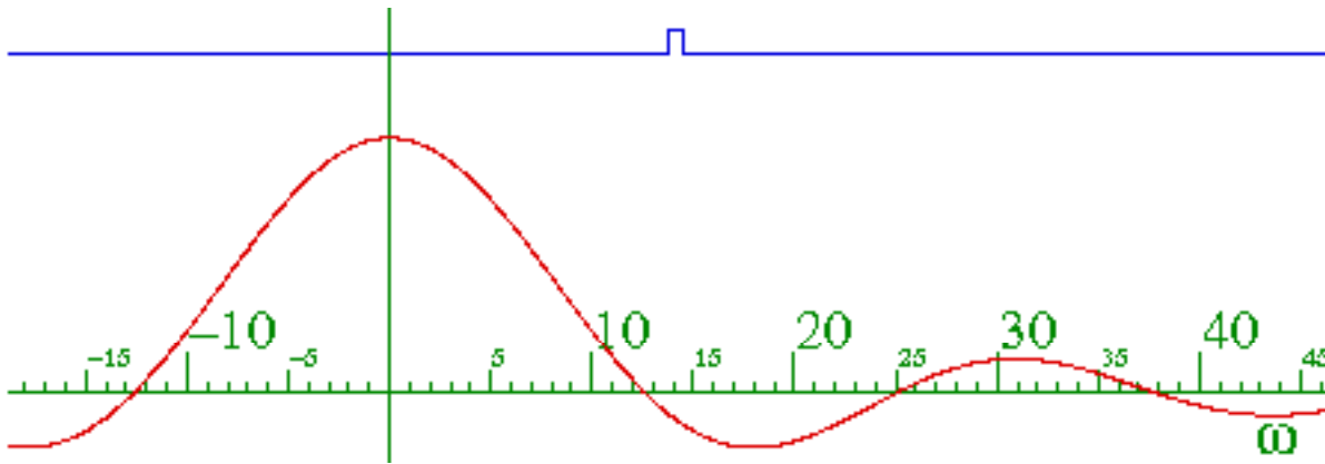
Fig. 3.6.7 Elementary diffraction function: Fourier transform of single half square wave.
