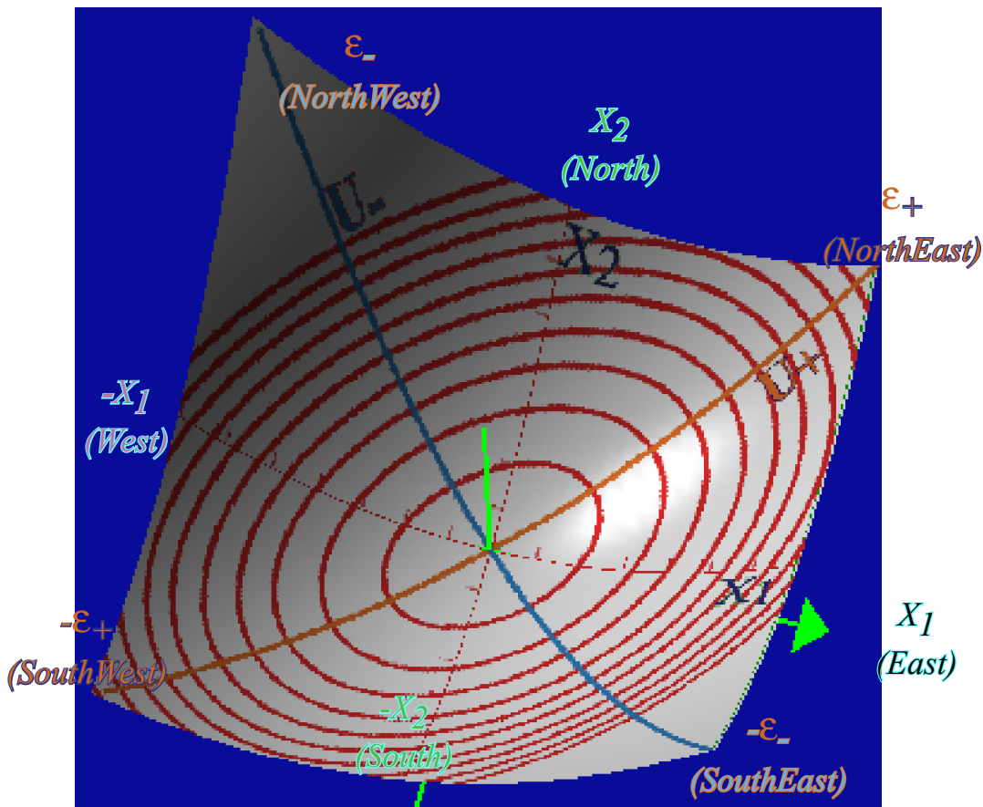
Fig. 3.3.4 Plot of potential function V(x_1, x_2) showing elliptical V(x_1, x_2) = const. level curves.
