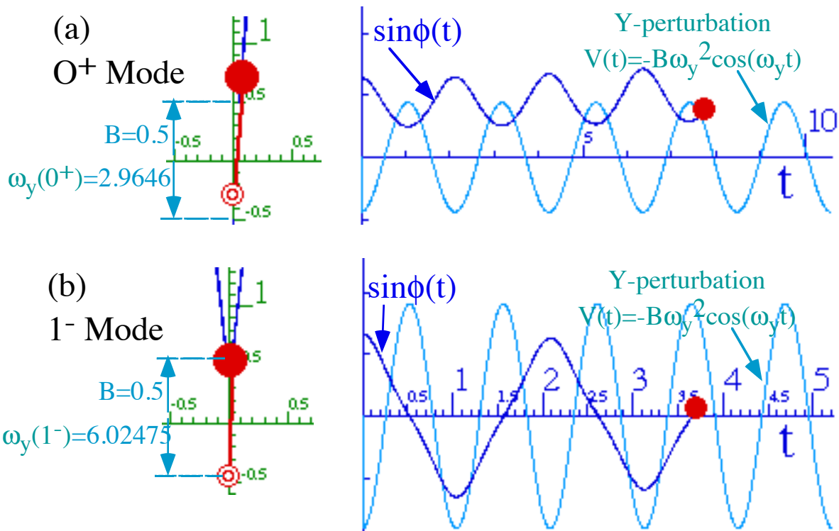
Fig. 3.7.3 Inverted Modes (a) Symmetric (one sided) 0^+ mode, (b) Anti-symmetric 1^- mode .
