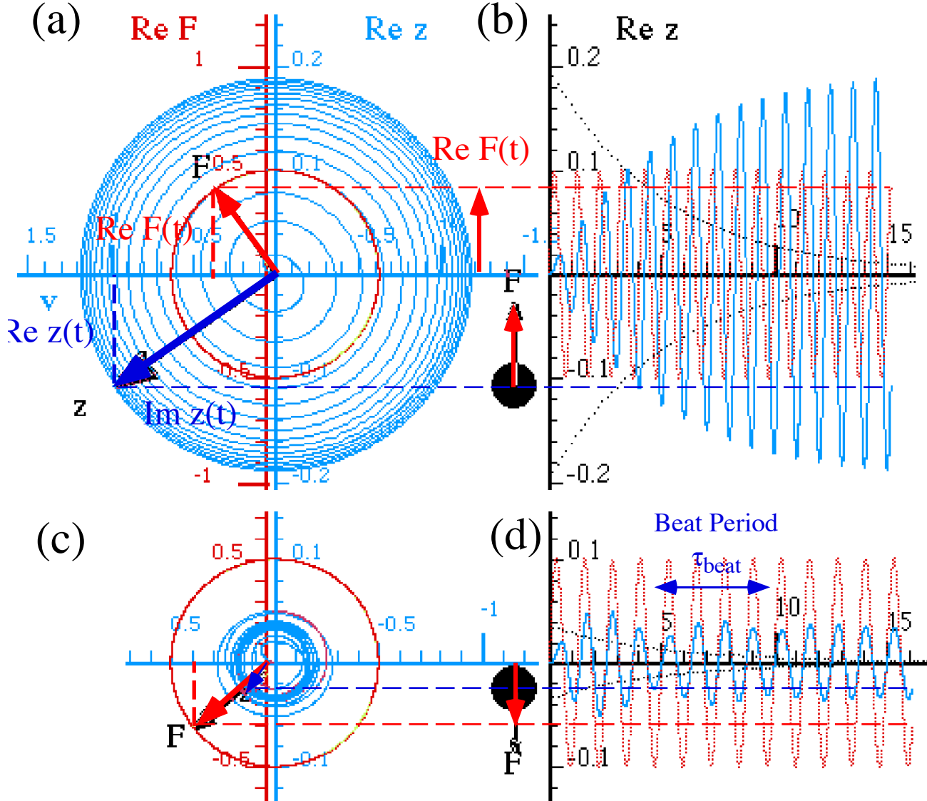
Fig. 3.2.8 On Resonance (a) Response z -phasor lags \rho = 90^\circ behind stimulus F -phasor. ( \omega_s = \omega_0 = 2\pi and \Gamma = 0.2 ). (b) Time plots of Re z(t) and Re F(t)
