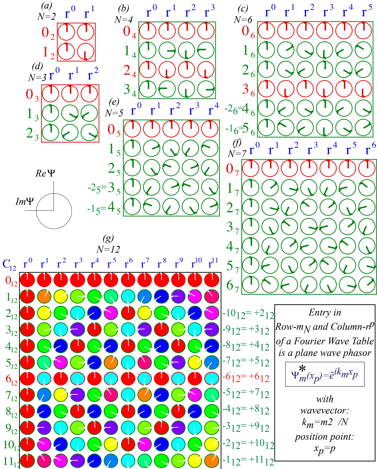
Fig. 3.8.6 Discrete wave phasor or Fourier transform tables for N=2,3,4,5,6,7 , and 12 .
