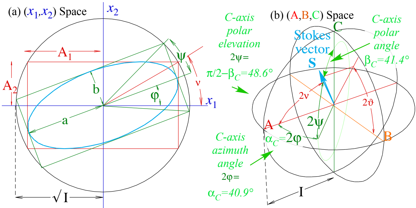
Fig. 3.4.4 Polarization described by (a) circular-RL bases and (b) C -axis polar angles of Stokes vector.
