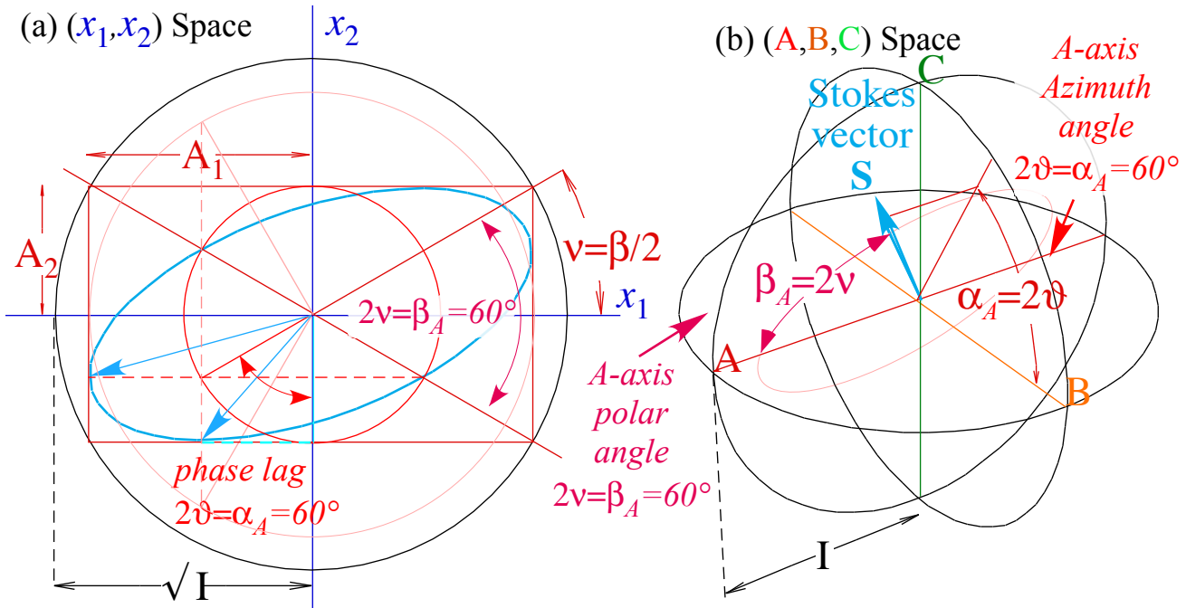
Fig. 3.4.3 Polarization described by (a) plane- x_1x_2 bases and (b) A -axis polar angles of Stokes vector.
